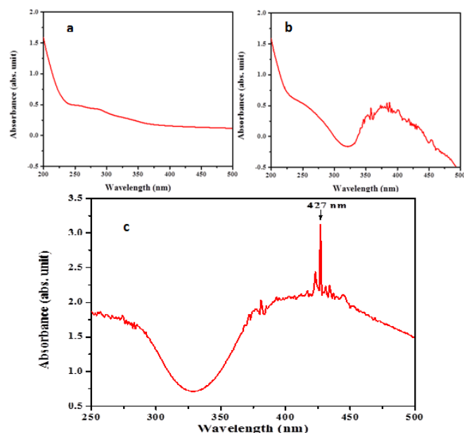
Figure 2. UV/ Vis spectra of mucilage samples; (a) Purified (b) Modified (c) Silver nanoparticles formulation.
