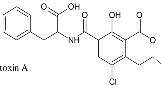
Figure 1. Structure of Ochratoxin A.
