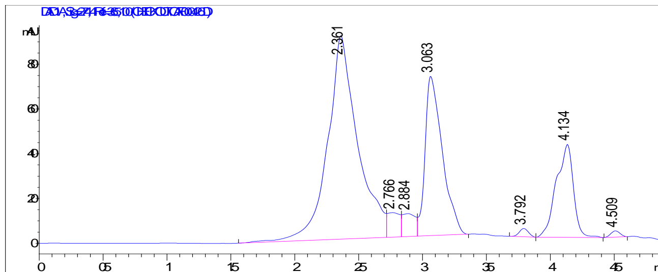
Figure 3. Chromatogram of Ochratoxin.
