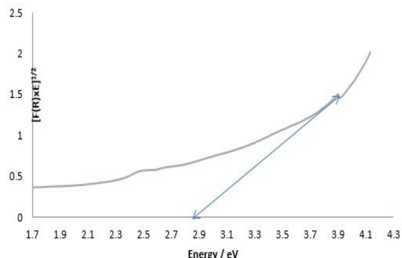
Figure 4. Bandgap energy of \text{Fe}^{3+} -5-ZnO sample.
