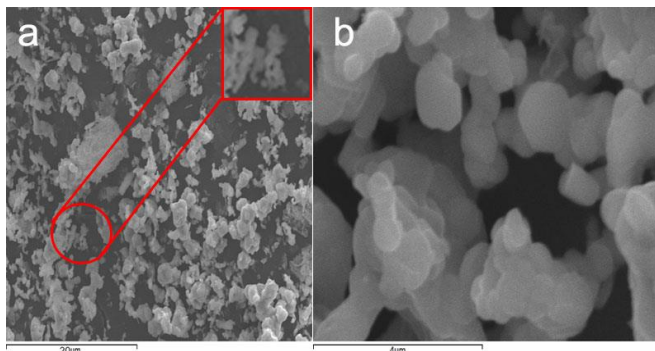
Figure 2. Images of SEM a) \text{Fe}^{3+} -5-ZnO nano discs at 5KX b) agglomerated \text{Fe}^{3+} -5-ZnO nano discs at 25 KX.
