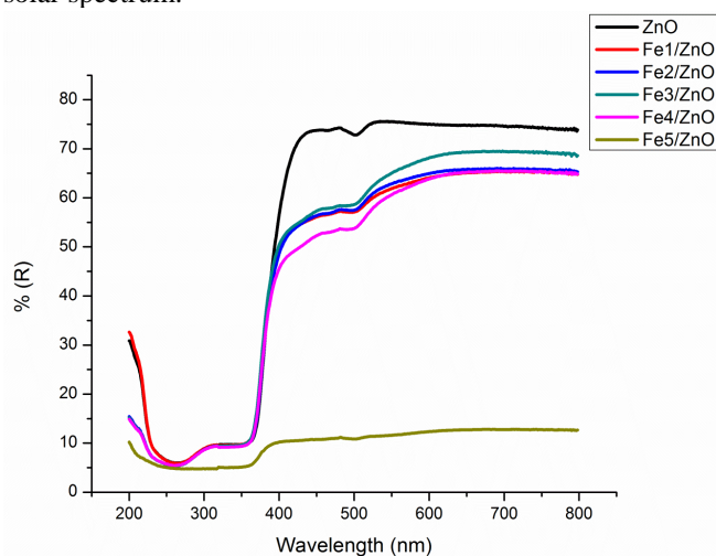
Figure 3. Comparison of diffused reflectance spectra of undoped and \text{Fe}^{3+} -doped ZnO.
