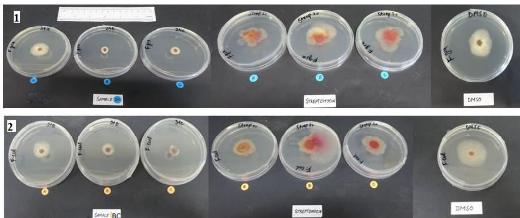
Figure 1. In-vitro effect of selected essential oils composition of C. aurantium , C. paradisi , C. sinensis against Fusarium graminearum (1) and Fusarium culmorum (2) at 4 days of incubation using poisoned food technique.
