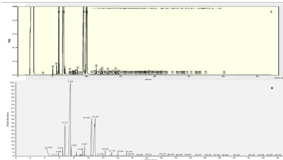
Figure 2. Typical GC-FID (A) and GC-MS (B) chromatogram of C. aurantium essential oil.
